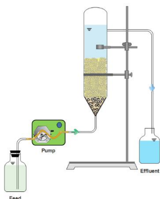
Figure 1: Schematic view of reactor
