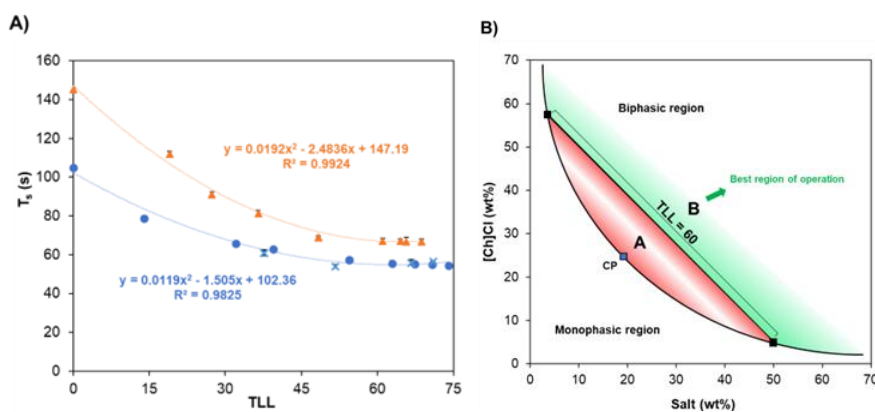
Figure 1: T_s values as a function of TLL at 25 °C (A) (● – mixture points of [Ch]Cl/ K_3PO_4 ; (▲ – mixture points of [Ch]Cl/ K_2HPO_4 ; × – mixture points from Shahriari et al. 2 ; and generic best region of operation for [Ch]Cl-based ABS. Adapted from Jorge et al. 1 .
