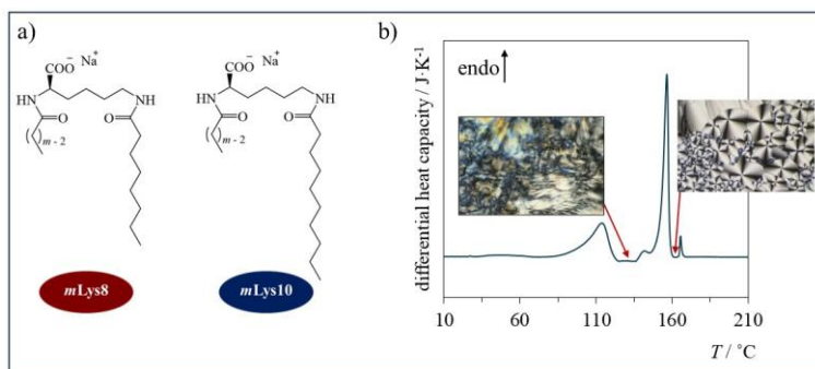
Figure 1: a) Molecular structure of the mLys n lysine-based surfactants; b) DSC thermogram of 12Lys8 surfactant and illustrative micrographs of the birefringent smectic A phase textures obtained by polarized light microscopy.
