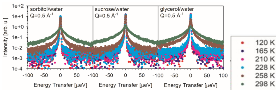
Figure 1: Examples of QENS spectra with BASIS instrument for 70% PHC+30% water at 120K to 298K.
