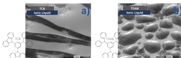
Figure 1: SEM micrographs exhibiting OSCs' crystalline growths when deposited over ionic liquids. a) 1,3,5-Tris(N-carbazolyl)benzene (TCB) deposited over [C_8C_1Im][NTf_2] , b) 1,3,5-Tris(diphenylamino)benzene (TDAB) deposited over [C_8C_1Im][NTf_2] .
